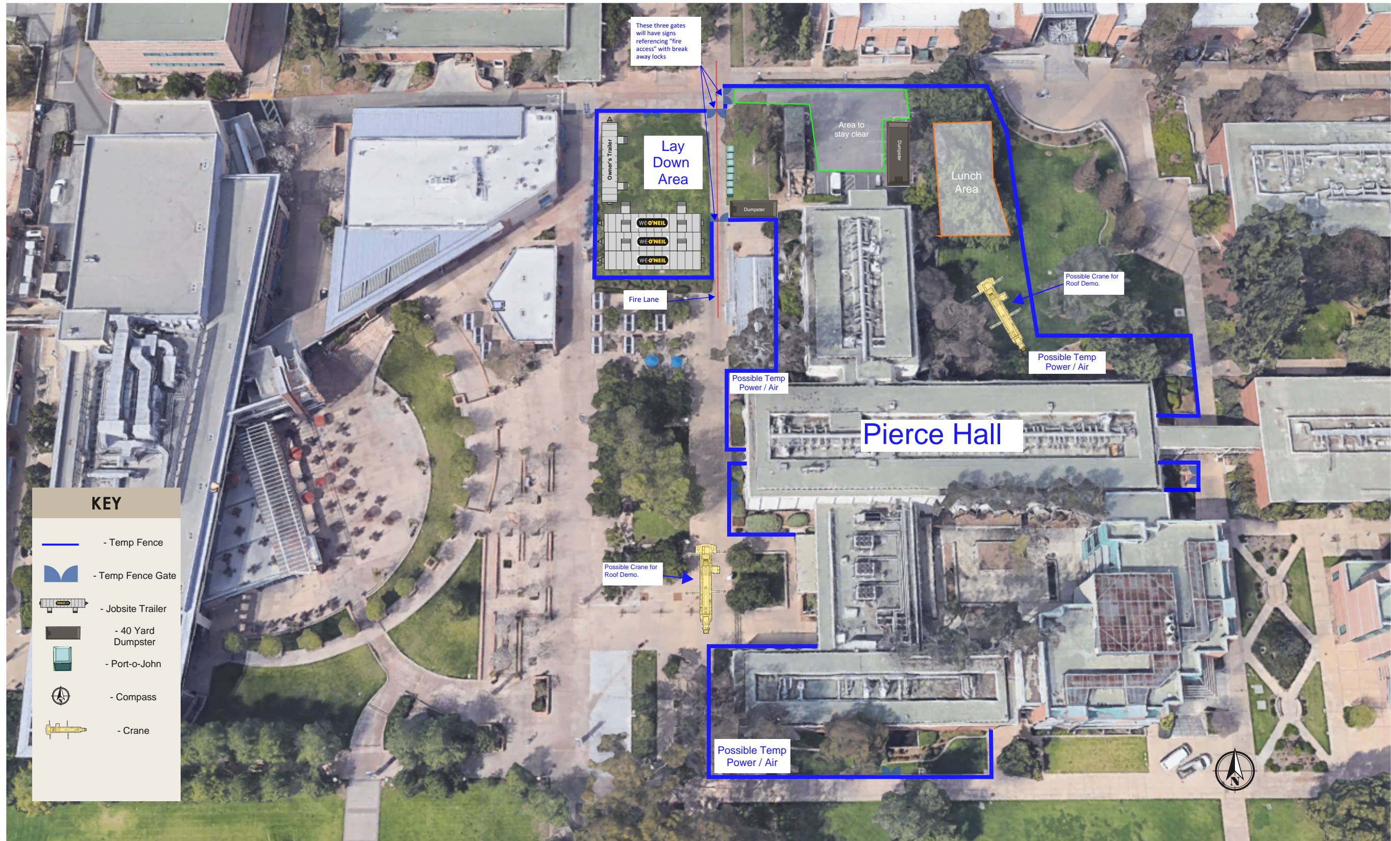
Site Logistics Plan
