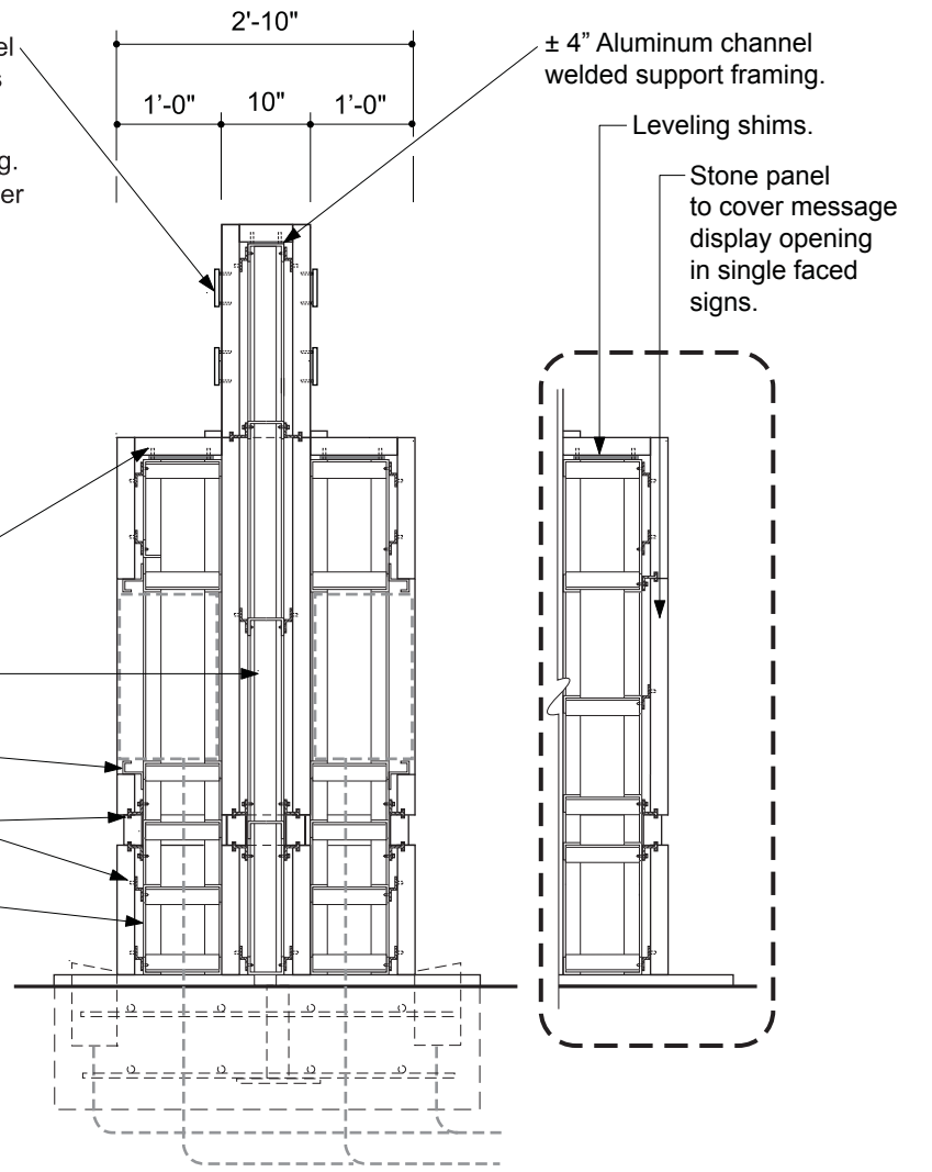
DOUBLE SIDED SECTION 1/2" = 1'-0" A
