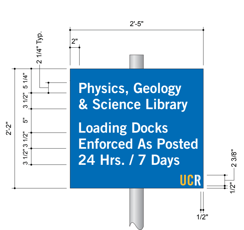
5-LINE CONDITION | 1" = 1'-0"
