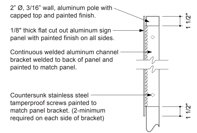
SIDE VIEW | 1 1/2" = 1'-0"
